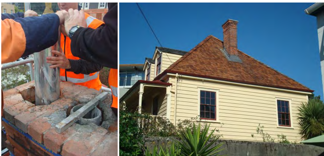
The chimney at Nairn Street Cottage has been fitted with a new structural chimney liner and fixed back to a new roof diaphragm. Photos: Hawkins Construction NI Limited & Carlos Gonzales, WCC Architectural Services.
