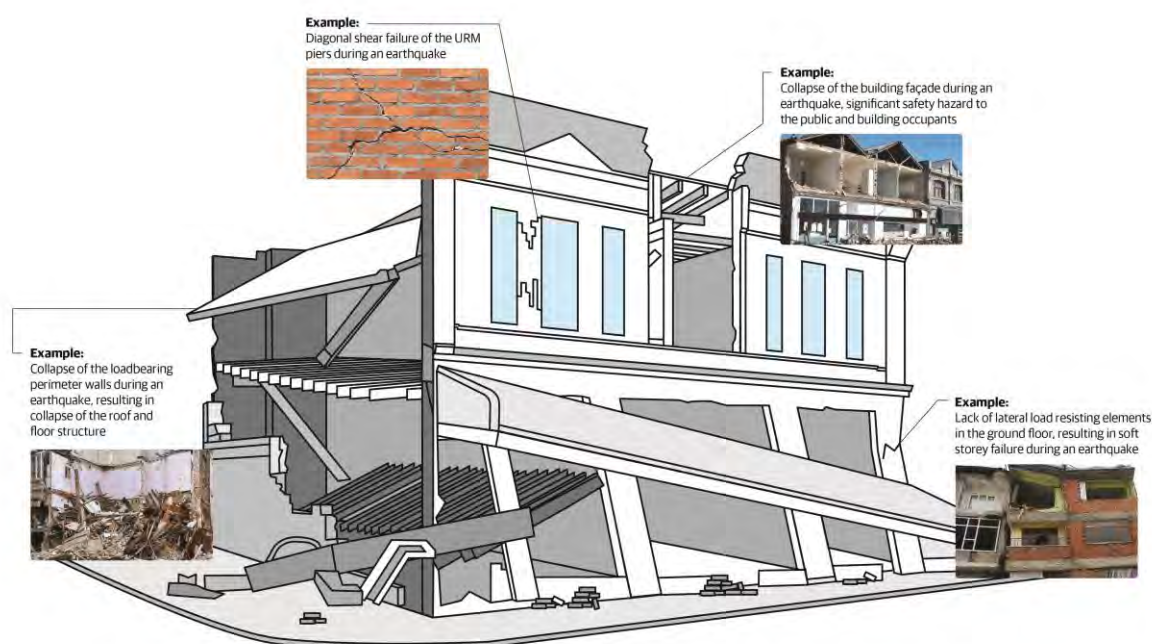
Figure 2: Common issues for a typical URM commercial building during an earthquake.
